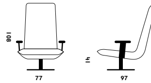
EL. 118M / 118MA (armrest)
